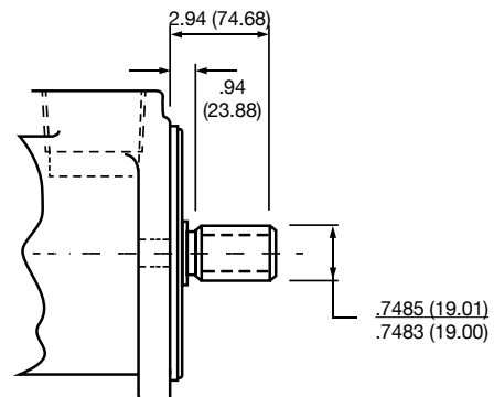
No. 11 Splined Shaft, 9 Tooth
